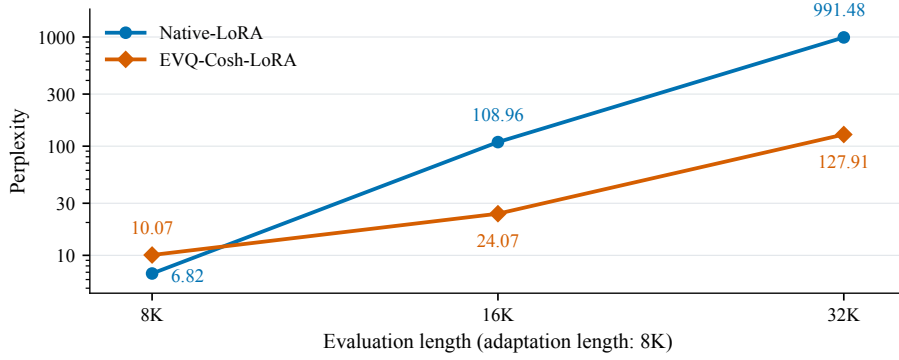
Figure 3: Cosh allocation improves extrapolation under matched adaptation. Llama-3-8B arms share an 8K, 300-step LoRA protocol on 24 text packs. PPL is the exponential of equal-domain mean NLL.
