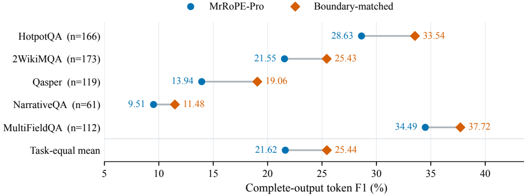
Figure 4: Intermediate-band redistribution improves OLMo natural QA. Complete-output token F1 on untruncated long inputs ( s = 4 ). Sample counts shown by task; final row averages task means.
