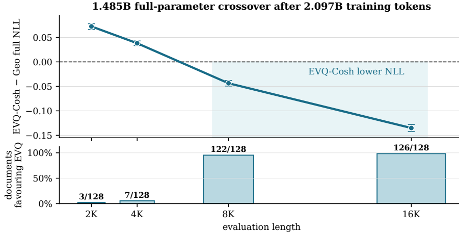
Figure 8: Full-parameter scale evidence crosses beyond the training window. The 1.485B Geo and EVQ-COSH arms start from the same public initialisation and follow the same scientific recipe for 2.097B tokens. Error bars are paired bootstrap intervals over the same 128 held-out documents, conditioned on this trained pair; the lower panel gives the document count favouring EVQ-COSH at each length.
