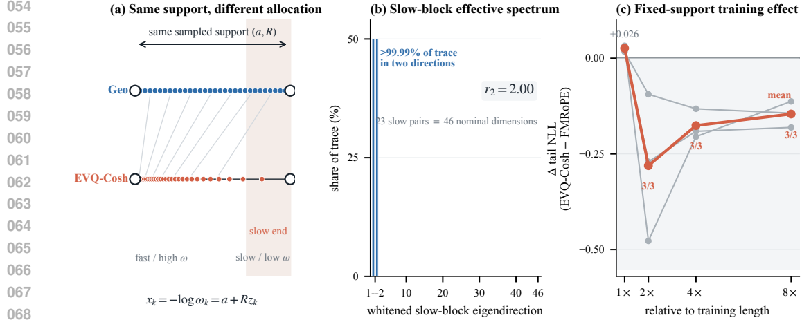
Figure 1: A fixed nominal rotary budget can realise different effective positional bases. (a) Geo and anchored EVQ-COSH share K=32 , operator, endpoints, and log-span; z changes the phase-scale density. (b) Exact geometry: for standard RoPE at L=4096 , b=5 \times 10^5 , and K=64 , the 23 pairs with \omega L \leq 1 place more than 99.99% of their block-whitened trace in two eigendirections and have r_2=2.00 under the stated uniform separation prior. (c) Causal identification: moving only 30 interiors at fixed support improves every tested OOD length in all three seeds.
