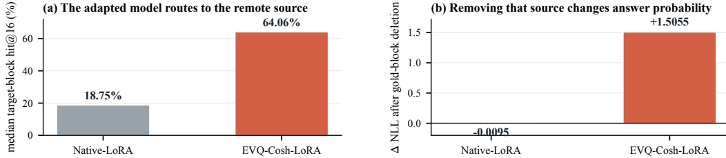
Figure 3: Matched adaptation converts the new basis into causal remote-source use. On ten frozen true-16K cases, (a) median target-block hit@16 is measured over 32 retrieval heads; (b) answer-side decode attention to the remote gold block is then removed from every head while preserving prompt tokens, rotary KV indices, and block geometry. The +1.5055 NLL change shows that the adapted evq model’s answer probability depends on that source, while the Native control is essentially unchanged. These are routing and teacher-forced probability endpoints, distinct from autoregressive task accuracy (App. E.3).
