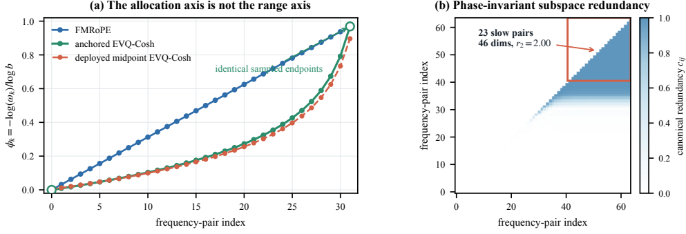
Figure 3: Where a finite frequency table spends its budget. (a) At K=32 , Cosh concentrates interior channels toward the fast end while endpoint normalisation preserves sampled support; the deployed midpoint table is shown separately. (b) For standard RoPE at L=4096 , b=5 \times 10^5 , and K=64 , phase-invariant full-subspace redundancy concentrates in the 23 pairs with \omega L \leq 1 .
