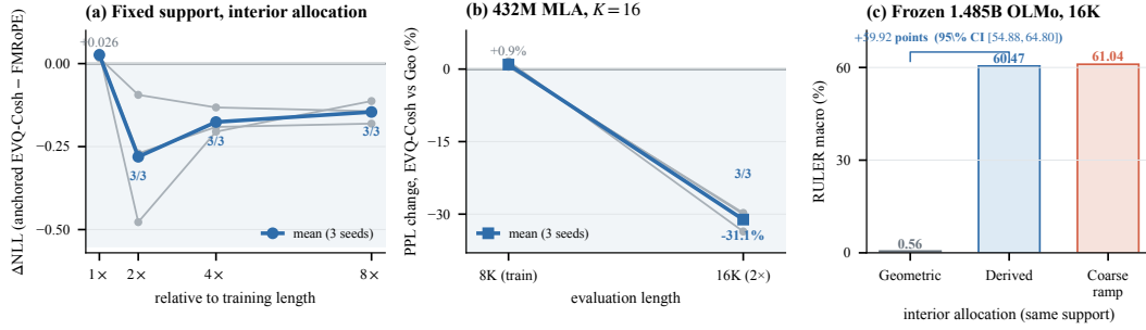
Figure 1: Interior allocation is identifiable and consequential. (a) Moving only interior frequencies improves every OOD length in all three 151.9M training seeds. (b) In a three-seed 432M MLA setting with only K=16 rotary pairs, the in-window cost is small and 16K PPL falls by 31.1%. (c) At fixed support, amplitude, checkpoint, data, and decoder, changing only z raises released-model 16K RULER macro from 0.56% to 60.47%; a coarse ramp matches the detailed profile.
