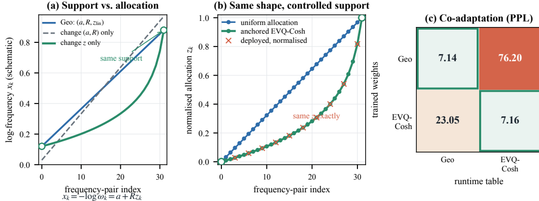
Figure 2: Support does not determine allocation. (a) Equation (1) separates support (a, R) from normalised interior allocation z . (b) Anchored EVQ-COSH and deployed midpoint EVQ-COSH have exactly the same z after support normalisation. (c) The table is learned with the weights: self-consistent pairs remain near PPL 7, while frozen post-hoc swaps fail.
