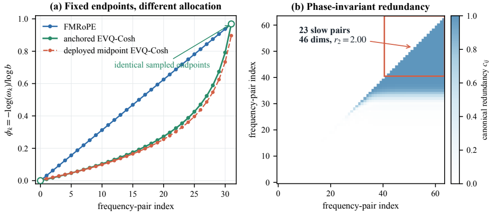
Figure 2: Where a finite frequency table spends its budget. (a) At K=32 , Cosh concentrates interior channels toward the fast end while endpoint normalisation preserves sampled support; the deployed midpoint table is shown separately. (b) For standard RoPE at L=4096 , b=5 \times 10^5 , and K=64 , phase-invariant full-subspace redundancy concentrates in the 23 pairs with \omega L \leq 1 .
