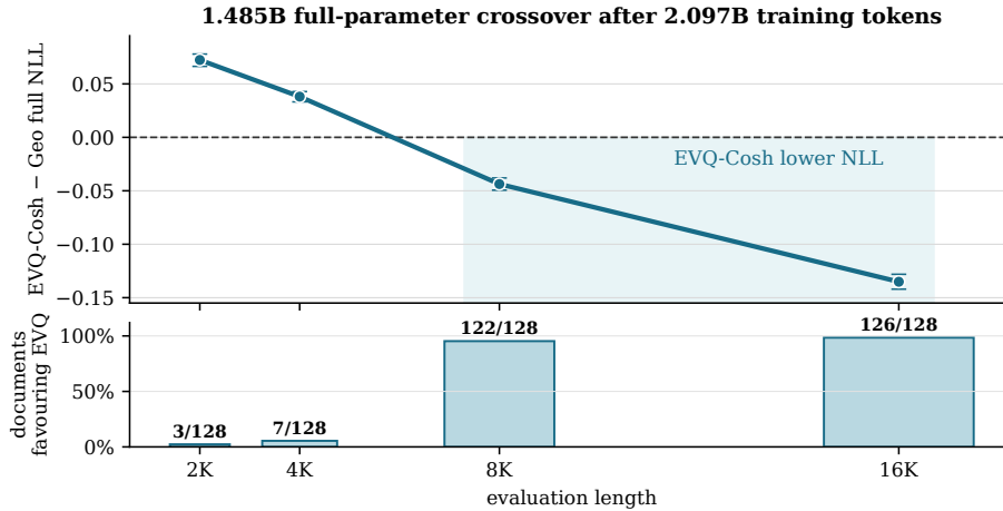
Figure 5: Full-parameter scale evidence crosses beyond the training window. The 1.485B Geo and EVQ-COSH arms start from the same public initialisation and follow the same scientific recipe for 2.097B tokens. Error bars are paired bootstrap intervals over the same 128 held-out documents, conditioned on this trained pair; the lower panel gives the document count favouring EVQ-COSH at each length.
