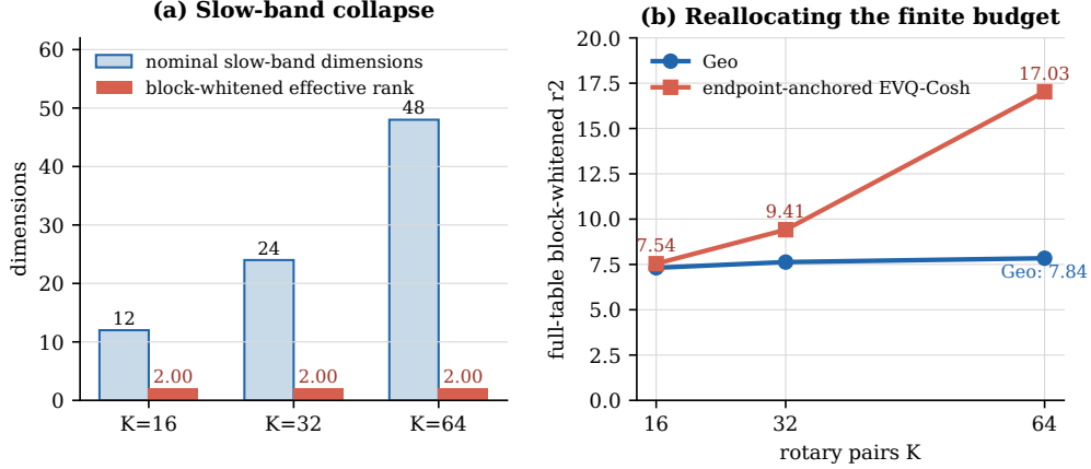
Figure 3: Spectral-budget anatomy across channel counts. Panel (a) uses the endpoint-inclusive diagnostic grid at L=4096 and b=500K : as K grows from 16 to 64, the nominal dimension assigned to pairs with \omega L \leq 1 grows from 12 to 48, while their phase-invariant effective rank remains approximately two. Panel (b) evaluates the complete fixed-endpoint table under the same uniform separation prior, using the zero-search reference \tau=2K/\sqrt{L} ; anchored EVQ-COSH spends progressively more of the available full-pair dimension than Geo as the budget grows.
