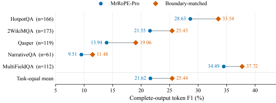
Figure 7: Intermediate-band redistribution improves OLMo natural QA. Complete-output token F1 on untruncated long inputs ( s = 4 ); sample counts shown by task, final row averages task means.
