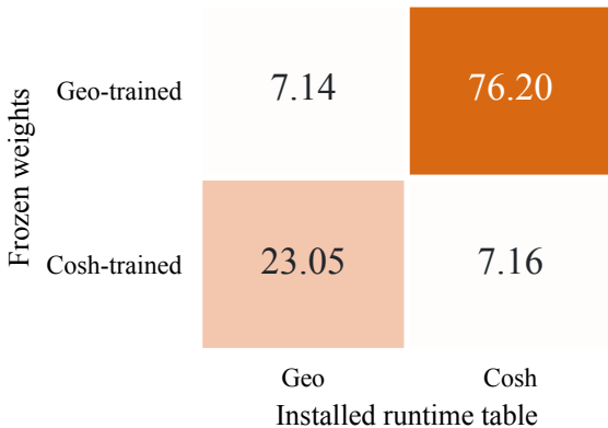
(a) 50M: perplexity
