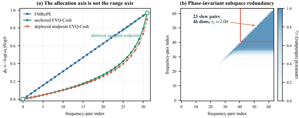
Figure 5: Where a finite frequency table spends its budget. (a) At K=32 , Cosh concentrates interior channels toward the fast end while endpoint normalisation preserves sampled support; the deployed midpoint table is shown separately. (b) For standard RoPE at L=4096 , b=5 \times 10^5 , and K=64 , phase-invariant full-subspace redundancy concentrates in the 23 pairs with \omega L \leq 1 .
