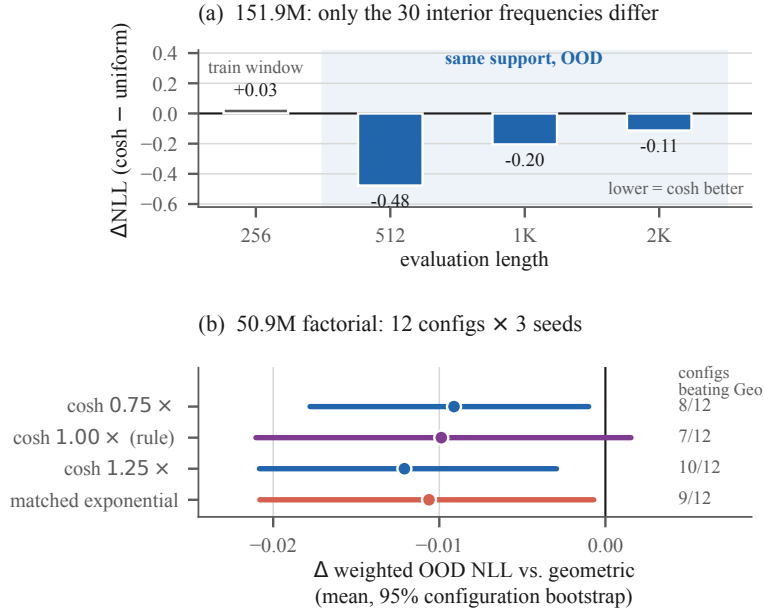
Figure 3: Allocation is identifiable. (a) With sampled extrema and log-span pinned, moving only the 30 interior frequencies incurs +0.033 NLL at the training length and changes OOD NLL by -0.478 / -0.205 / -0.113 (seed 42). (b) In a separate three-seed, 12-configuration factorial, two different analytic shapes favour non-uniform allocation in 10/12 and 9/12 configurations.
