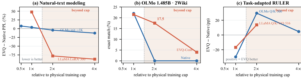
Figure 4: Training allocation shifts effective context across scale protocols. (a) Natural-text PPL crosses beyond the physical cap in a 1.485B from-initialisation trajectory and matched 8B LoRA. (b) Matched OLMo Q/K-only adaptation preserves 4K 2Wiki exact while transferring it to 8K/16K. (c) Separate task-adapted RULER runs show the same crossover. Protocols are not pooled; each panel reports its own matched comparison and seed scope (App. F).
