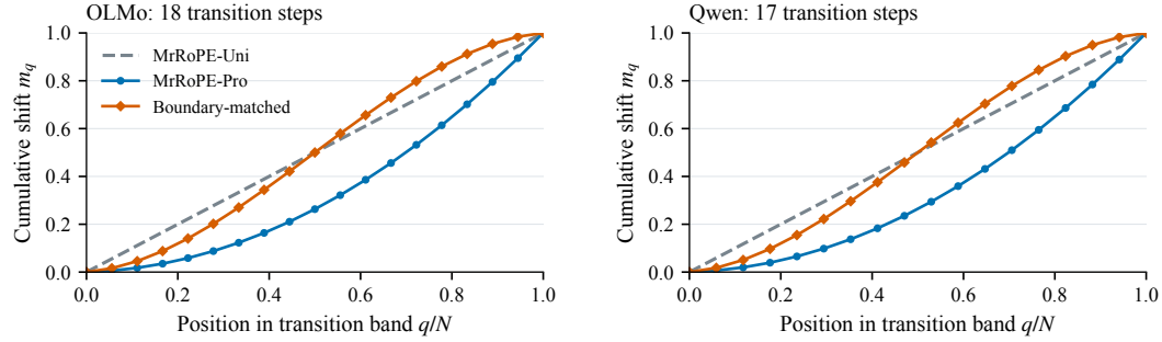
Figure 12: Intermediate-band exponent displacements. All three profiles have the same cumulative scale at the endpoints. BM redistributes the increments toward the middle of the transition band.
