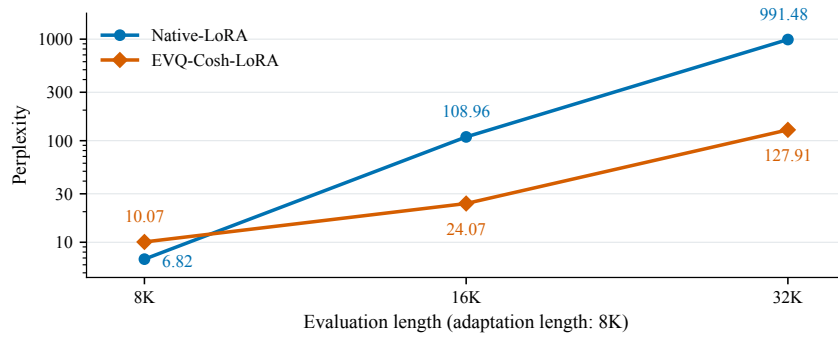
Figure 10: Cosh allocation improves extrapolation under matched adaptation . PPL is the exponential of equal-domain mean NLL.
