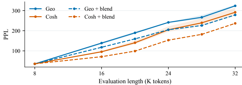
Figure 4: Cosh improves learning-time extrapolation. Three-seed mean PPL of the 432M MLA model. Solid curves use trained tables; dashed curves apply the same wavelength blend ( s = 4 ). Shading shows the three-seed range of the trained-table results.
