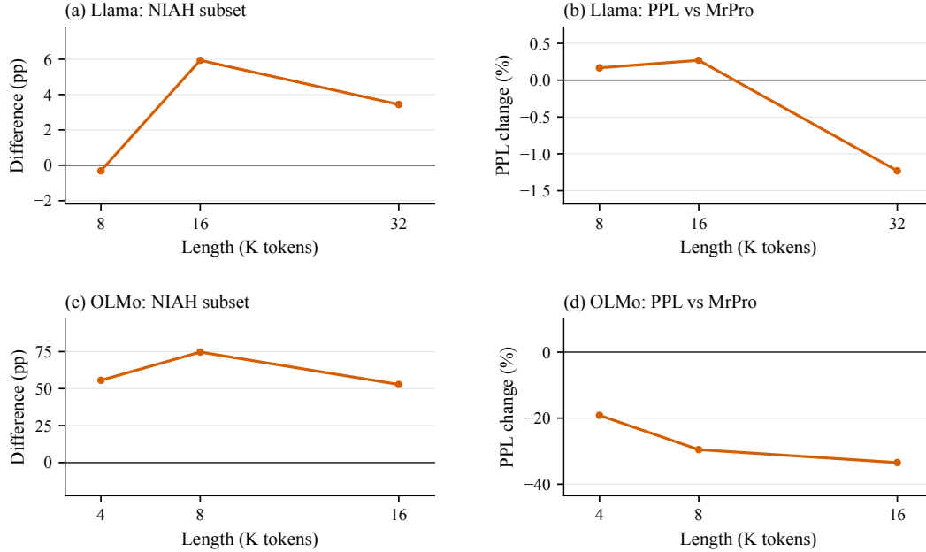
Figure 13: NIAH and language-modeling responses. NIAH is a subset of each model’s depth-balanced RULER-13 panel. Both columns show TailSpline relative to MrPro; PPL changes use each length’s absolute PPL. Llama’s 8/16K PPL slightly increases, while OLMo improves at every measured length. The panels have separate vertical scales.
