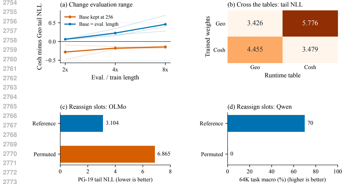
Figure 14: Three interventions distinguish the supplied spectrum from learned compatibility. (a) Range retargeting reverses the ordering of the same trained allocations; thin lines are three seeds and thick lines their means. (b) Crossed factor-four tables at 1K: rows are trained weights, columns runtime tables, and cells are mean tail NLL over two seeds and 32 anchors/seed. (c,d) Permuting interior frequency assignments preserves the final frequency multiset, endpoints and gain, but changes OLMo PG-19 tail NLL and Qwen 64K task macro (4 tasks, 20 rows/task). Each metric has its own axis. Joint Q/K compensation is the algebraic identity in (62), not a plotted recovery experiment.
