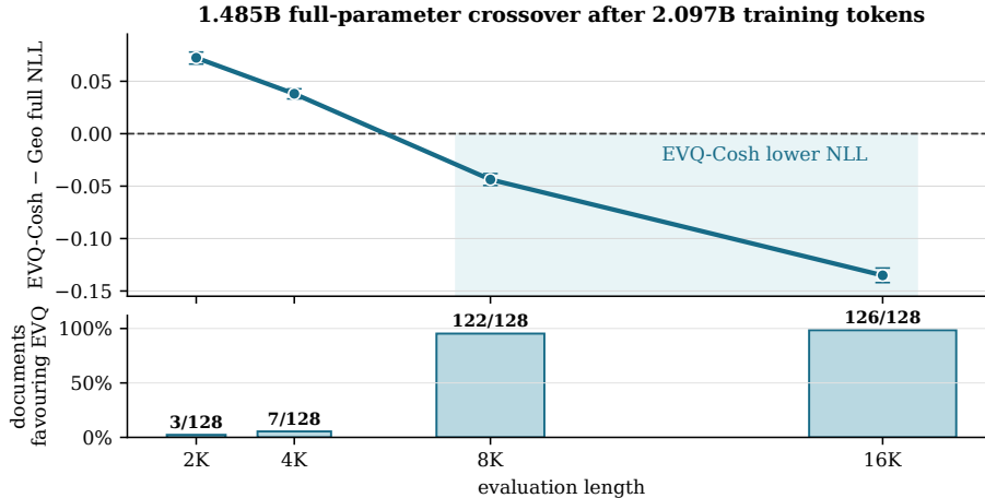
Figure 11: Full-parameter scale evidence crosses beyond the training window. The 1.485B Geo and EVQ-COSH arms start from the same public initialisation and follow the same scientific recipe for 2.097B tokens. Error bars are paired bootstrap intervals over the same 128 held-out documents, conditioned on this trained pair; the lower panel gives the document count favouring EVQ-COSH at each length.
