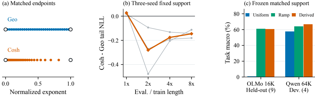
Figure 2: Interior allocation improves extrapolation and frozen tasks. (a) The matched geometric control (Geo) and anchored Cosh share both sampled endpoints and 32 rotary pairs. (b) Cosh-minus-Geo tail NLL at the training length ( 1\times = 256 ) and three extended lengths; thin lines show the three paired seeds, the thick line their mean. (c) OLMo’s nine held-out and Qwen’s four development tasks, with 20 inputs/task; arms share endpoints, amplitude, weights and inputs.
