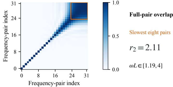
Figure 3: Slow rotary pairs share positional directions. Full-pair canonical overlap on the identification grid ( b = 256 , K = 32 , L = 256 ), under uniform separation measure on [0, L] . The outlined eight-pair block has effective rank r_2 = 2.11 despite \omega L \in [1.19, 4] .
