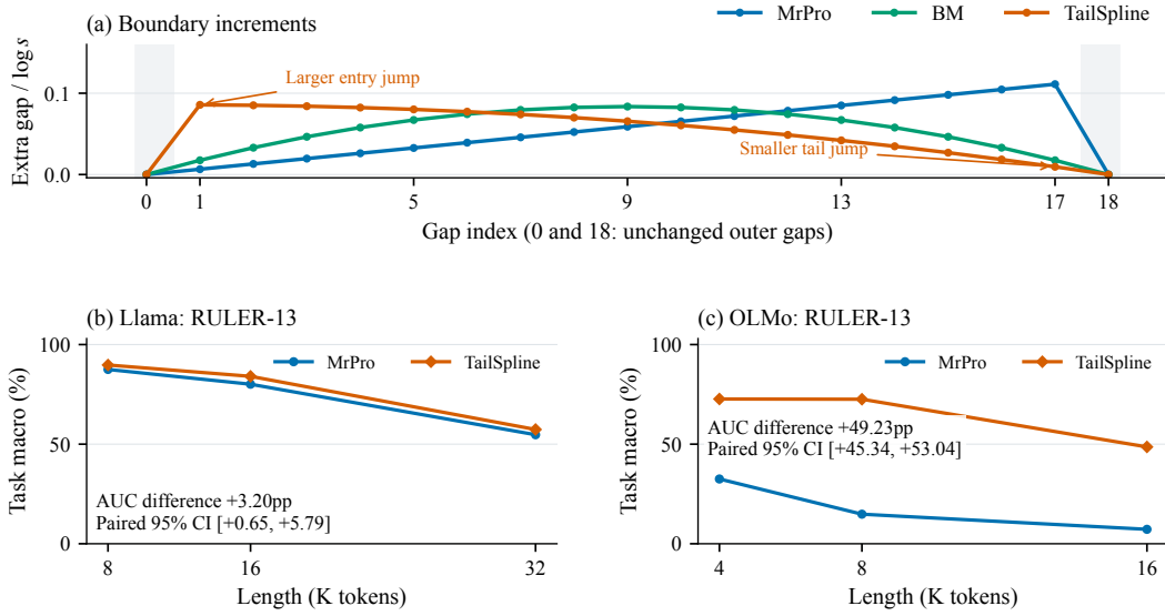
Figure 5: Boundary design improves frozen-model task scores. (a) At n = 17 , TailSpline trades a larger entry jump for a smaller tail jump. (b,c) Depth-balanced RULER-13 curves; annotations give log-length AUC differences and paired 95% intervals, not per-length intervals. Arms share band, endpoints, gain and inputs within each model. NIAH/PPL responses are in Appendix H.
