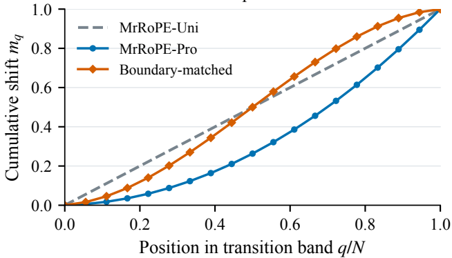
OLMo: 18 transition steps
