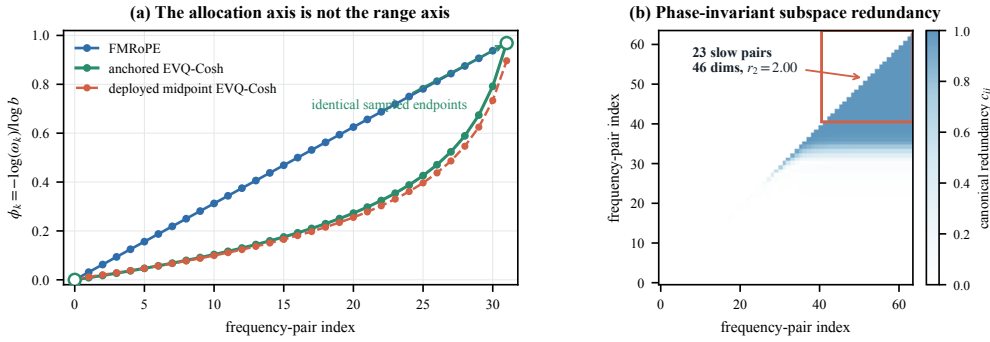
Figure 5: Where a finite frequency table spends its budget. (a) At K=32 , Cosh concentrates interior channels toward the fast end while endpoint normalisation preserves sampled support; the deployed midpoint table is shown separately. (b) For standard RoPE at L=4096 , b=5 \times 10^5 , and K=64 , phase-invariant full-subspace redundancy concentrates in the 23 pairs with \omega L \leq 1 .
