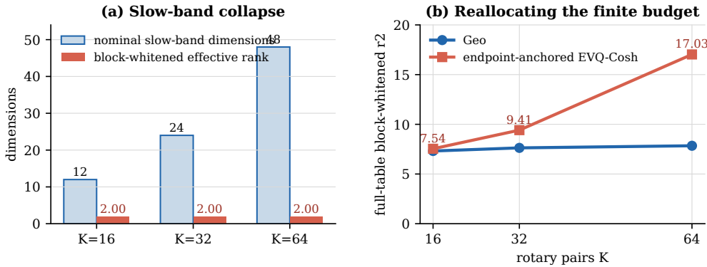
Figure 6: Spectral-budget anatomy across channel counts. Panel (a) uses the endpoint-inclusive diagnostic grid at L=4096 and b=500K : as K grows from 16 to 64, the nominal dimension assigned to pairs with \omega L \leq 1 grows from 12 to 48, while their phase-invariant effective rank remains approximately two. Panel (b) evaluates the complete fixed-endpoint table under the same uniform separation prior, using the zero-search reference \tau=2K/\sqrt{L} ; anchored EVQ-COSH spends progressively more of the available full-pair dimension than Geo as the budget grows. These are static positional-basis diagnostics; the trained effect is identified separately in App. C.
