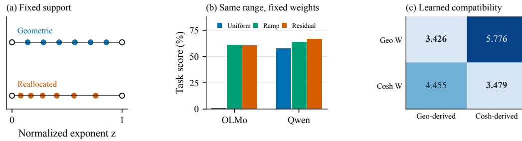
Figure 1: Frequency range leaves consequential allocation choices open. (a) Different interior placements share the same endpoints ( K = 8 illustration). (b) Frozen OLMo/Qwen models attain different task scores within a fixed range. (c) In paired training, each weight set favors the runtime table derived from its own allocation: two-seed mean tail NLL at 1K.
