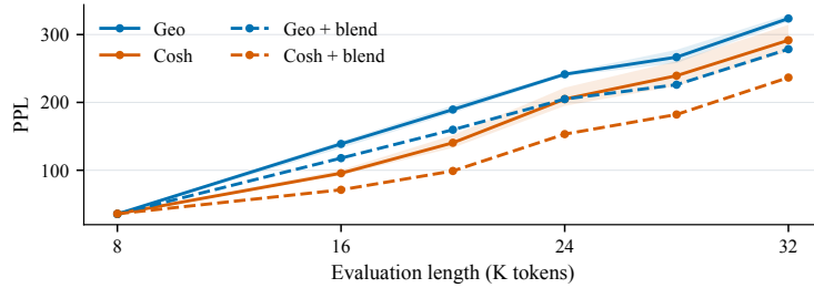
Figure 6: Cosh improves extrapolation across training seeds. Three-seed mean and range for the 432M MLA model; dashed curves use the common wavelength blend ( s = 4 ). Evaluation uses common text chunks.
