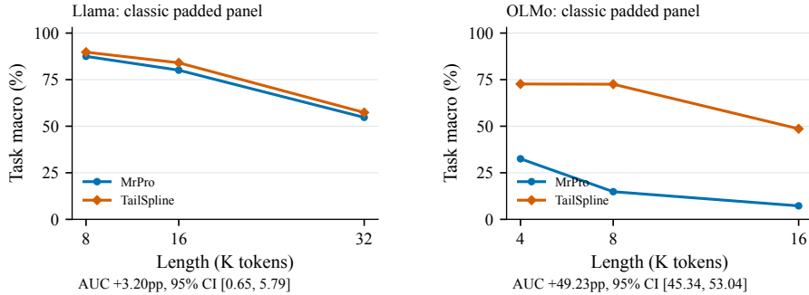
Figure 5: Classic task curves . Each model retains its own recorded depth-selected, prefix-padded protocol.
