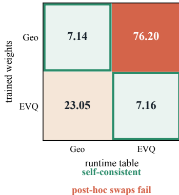
(c) Co-adaptation (PPL)
