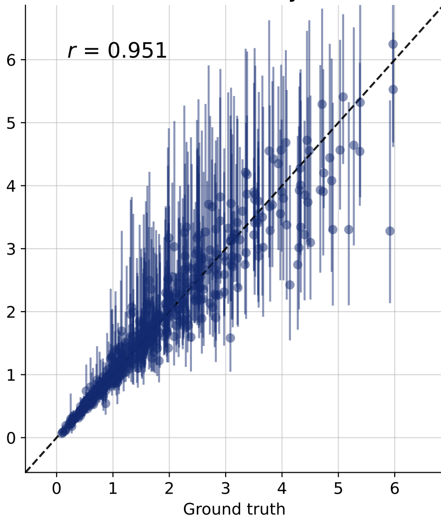
a (boundary)
