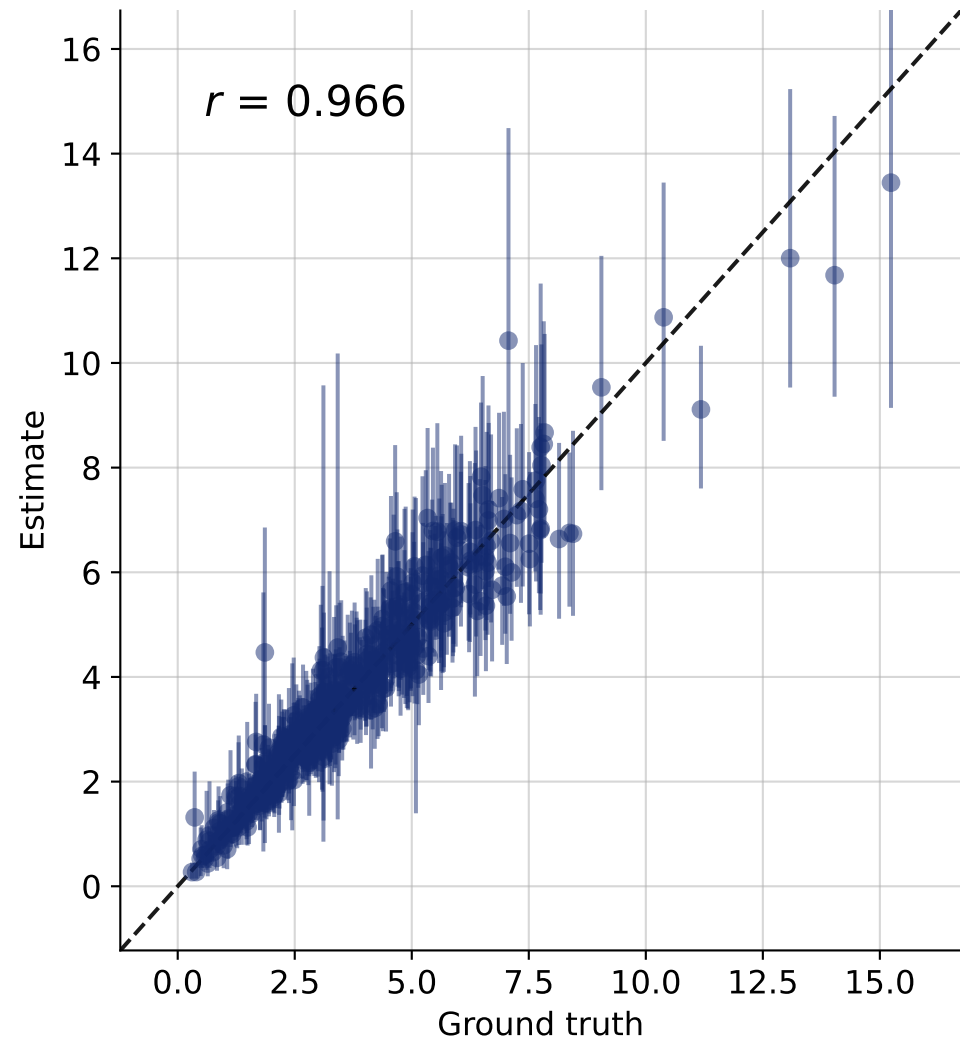
v (drift)
