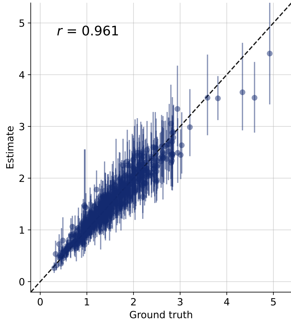
v (drift)
