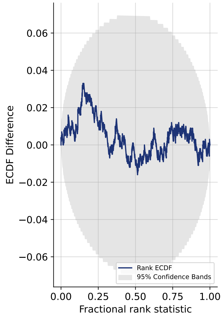
v (drift)
