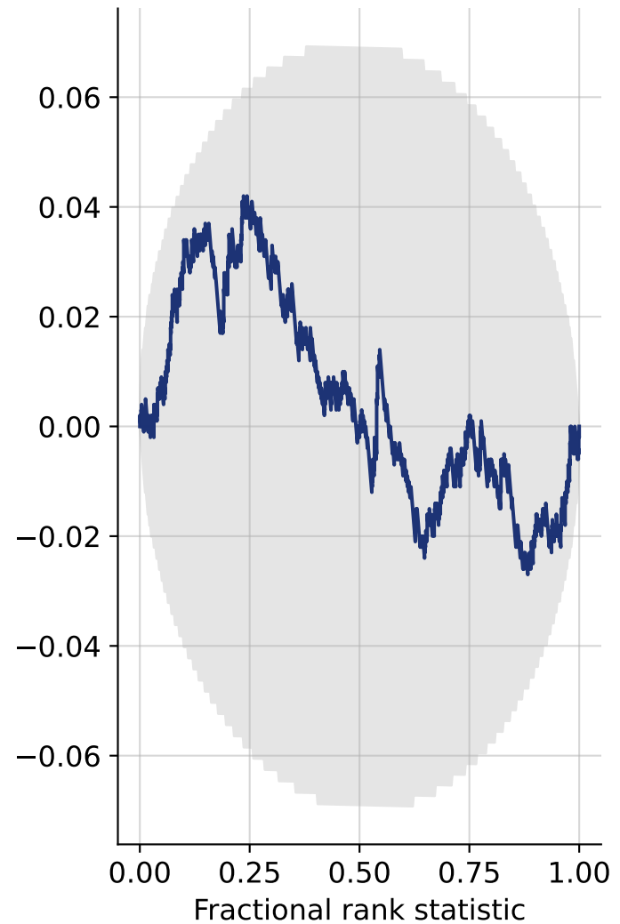
k (self-excitation)
