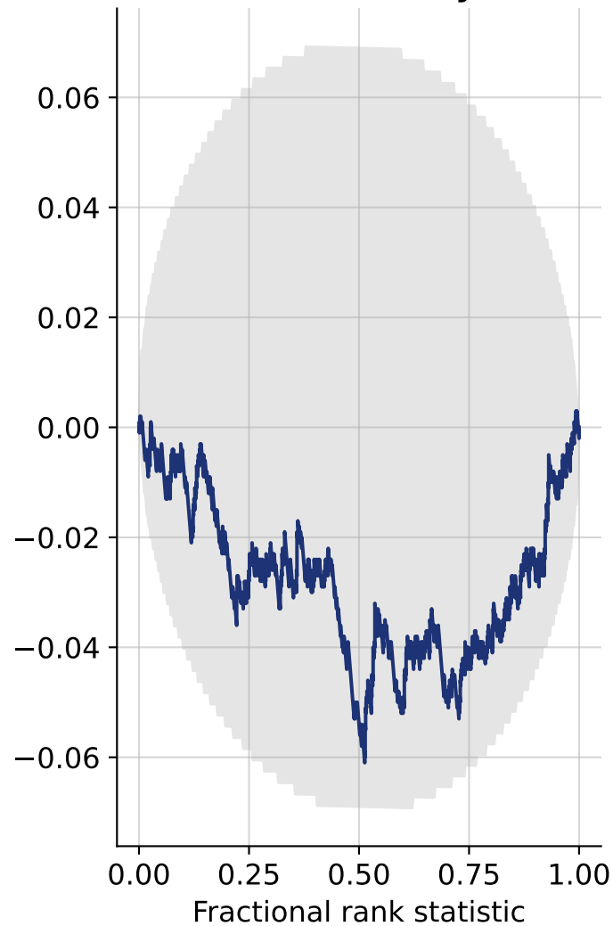
a (boundary)
