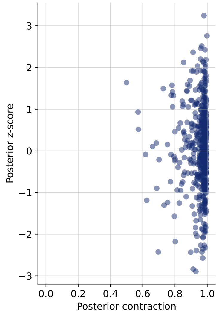
v (drift)
