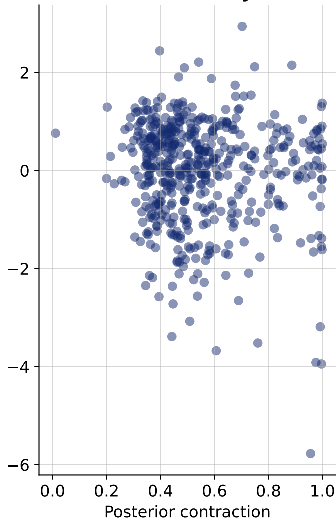
a (boundary)
