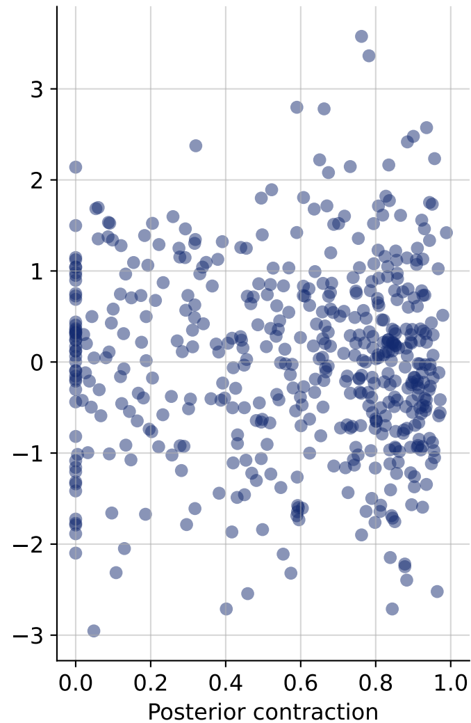
k (self-excitation)
