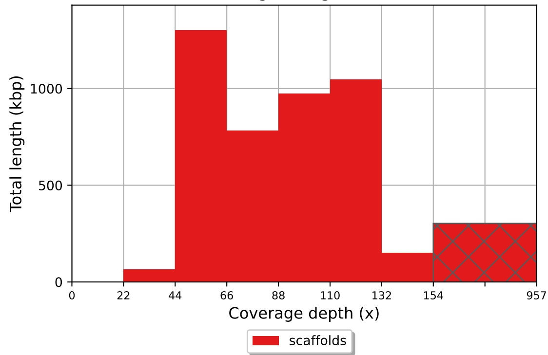
scaffolds coverage histogram (bin size: 22x)
