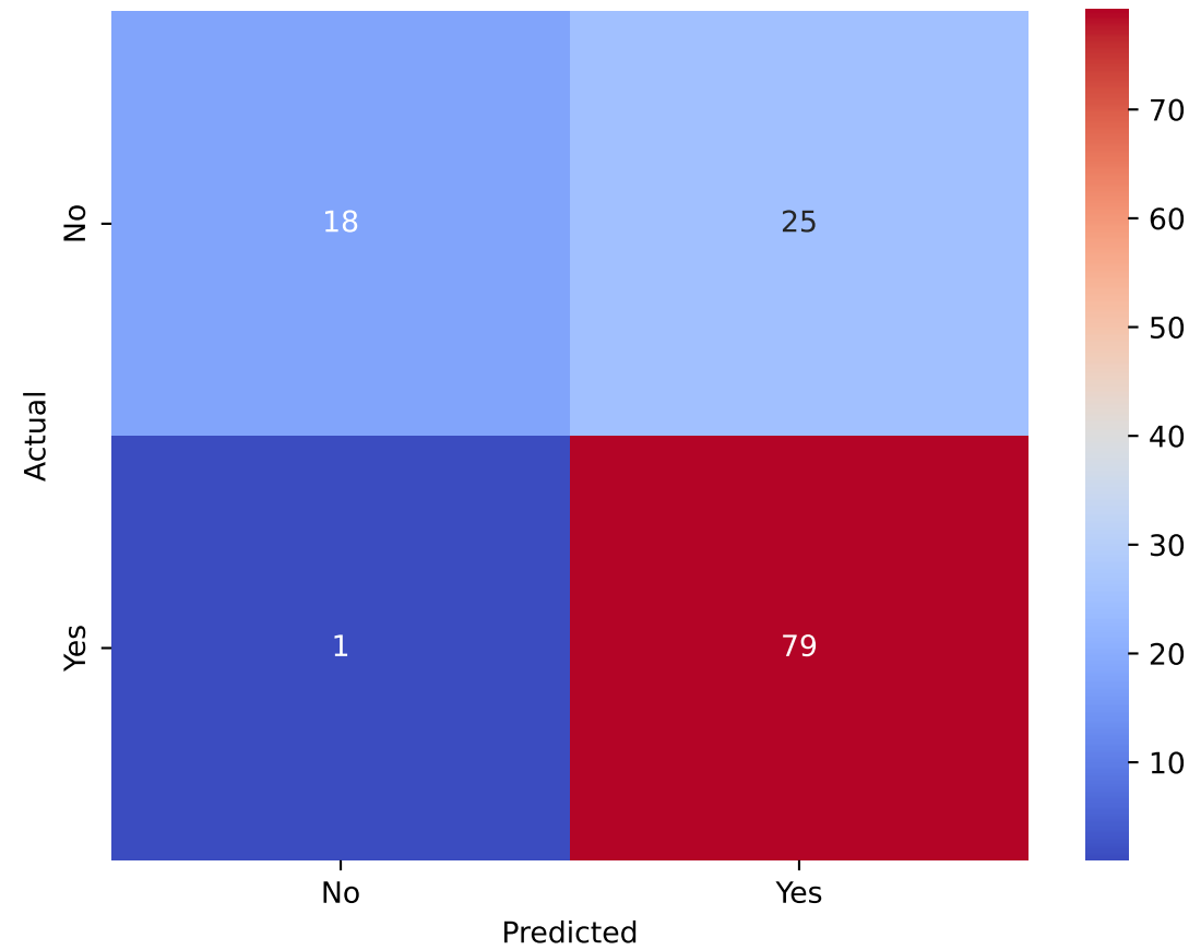
Confusion Matrix - Tuned XGBoost
