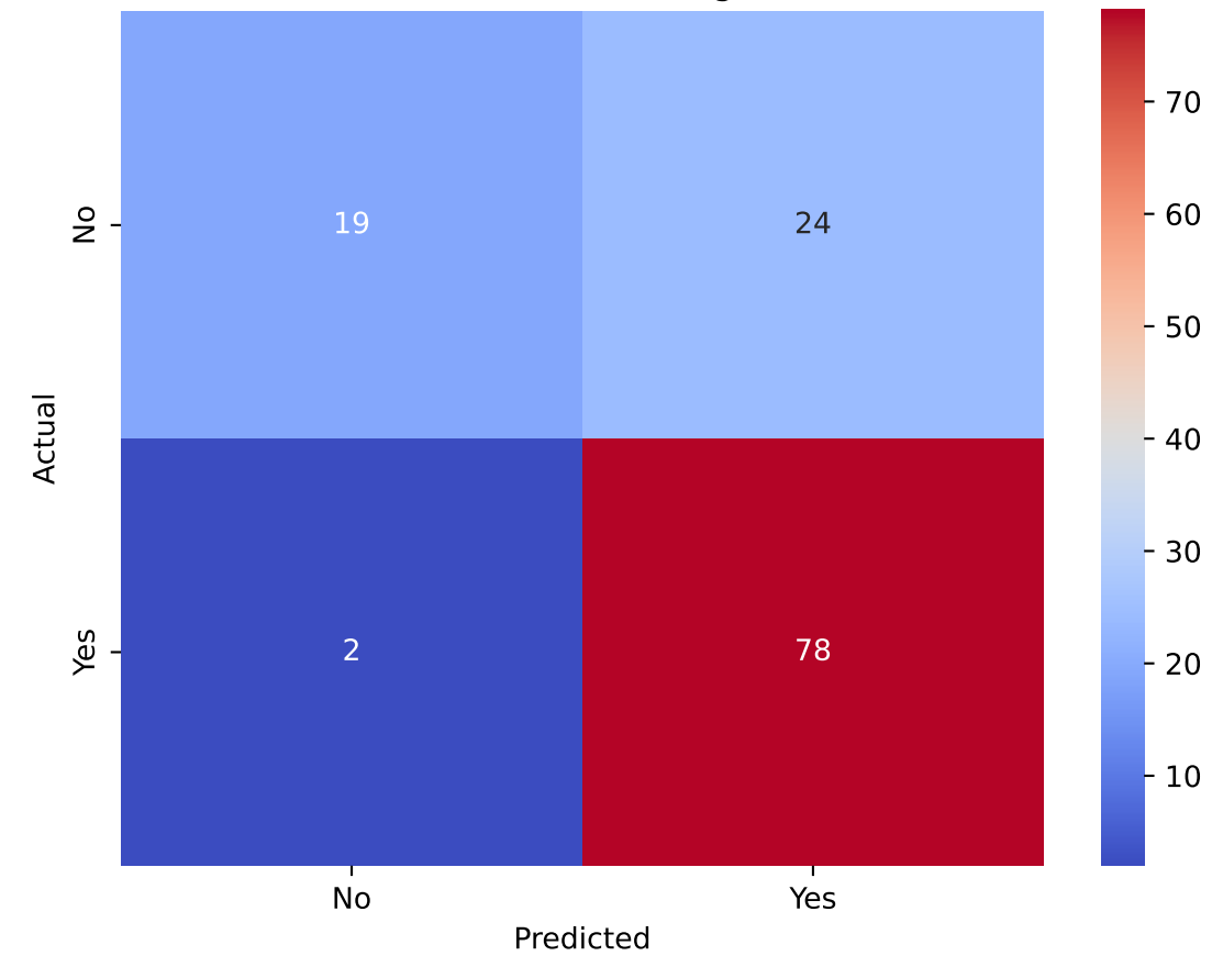
Confusion Matrix - Stacking Ensemble
