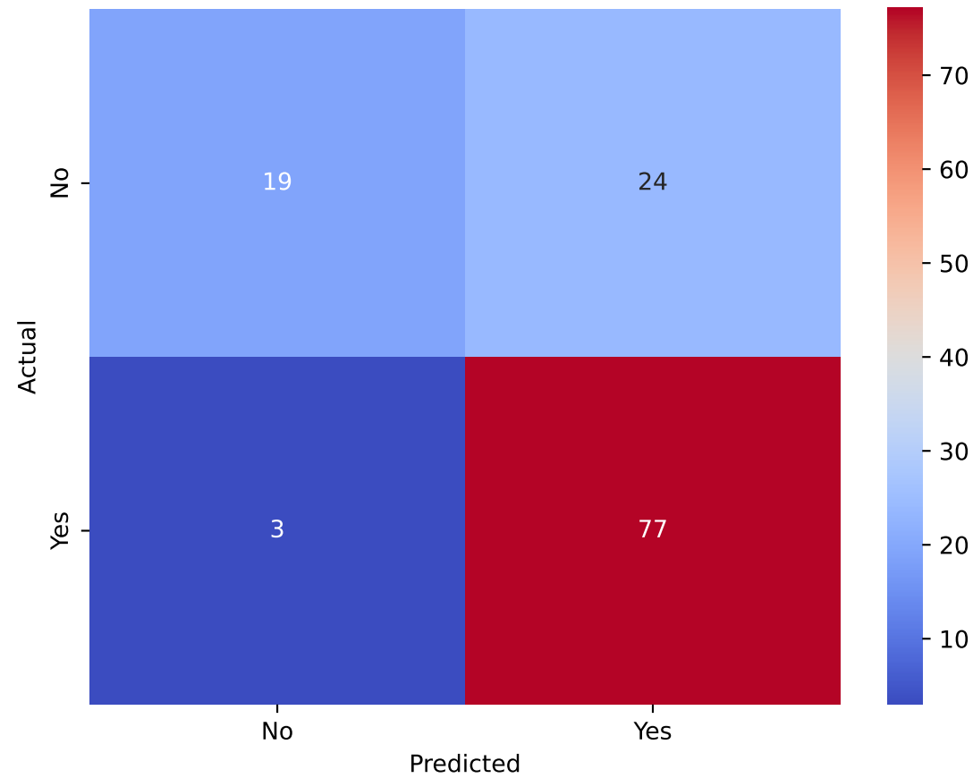
Confusion Matrix - Tuned Random Forest
