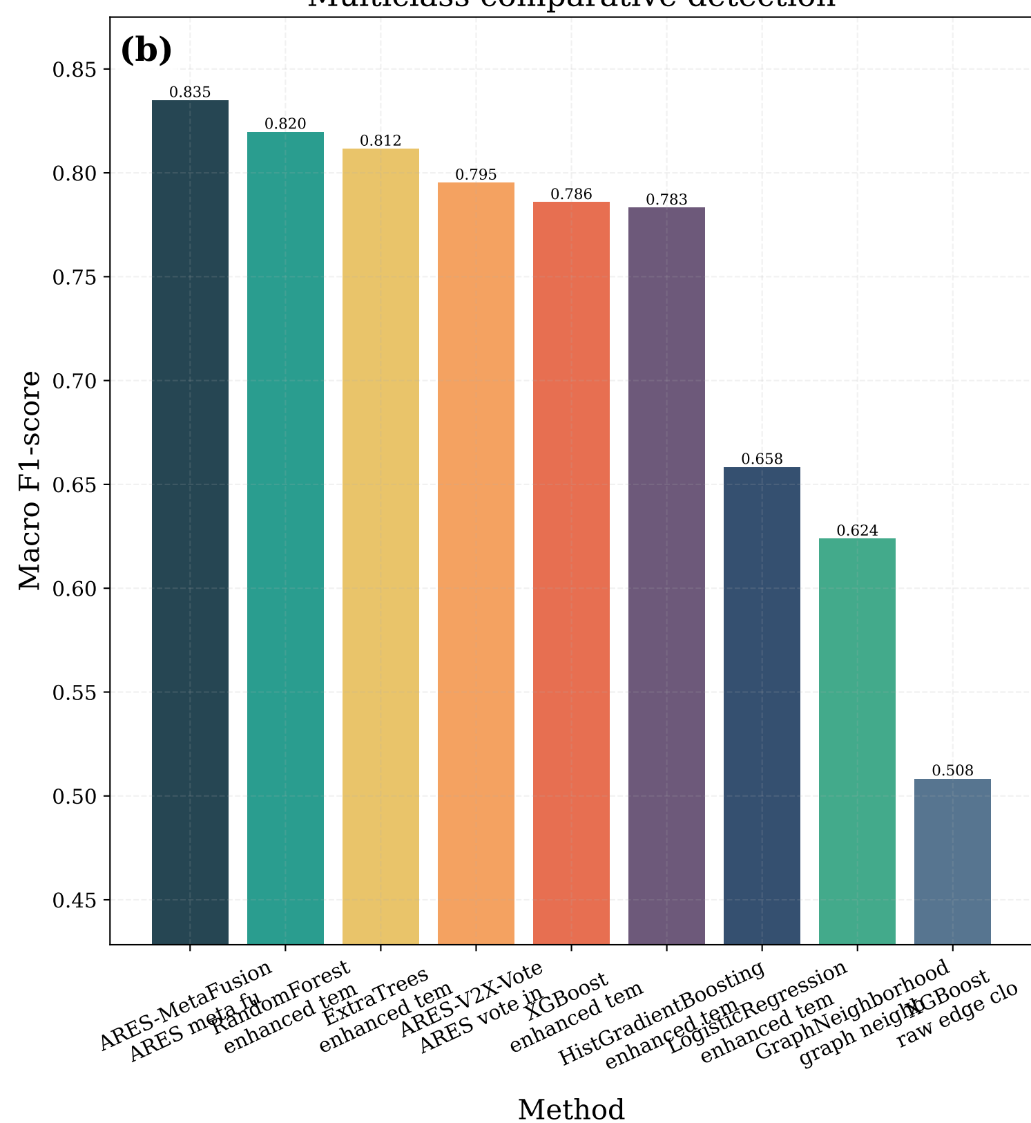
Multiclass comparative detection
