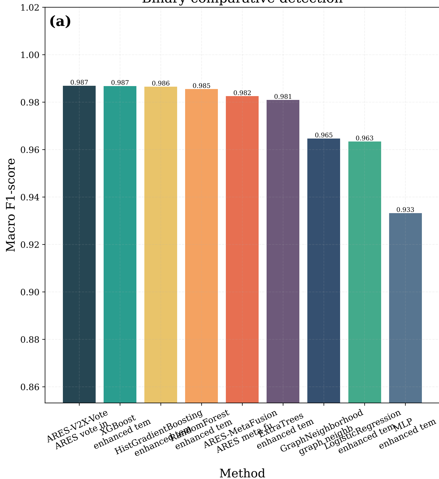
Binary comparative detection
