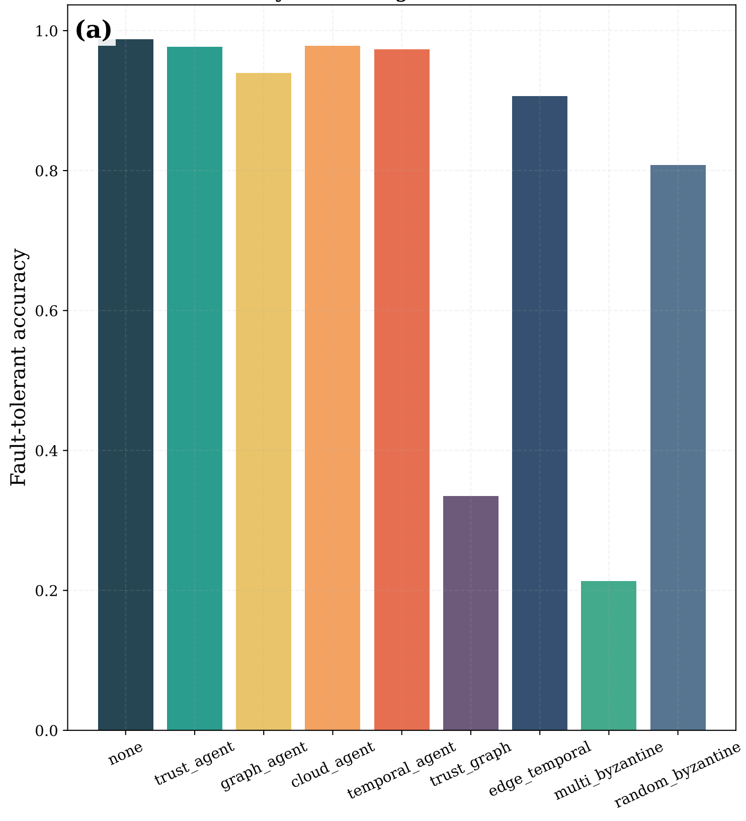
Byzantine-agent survival
