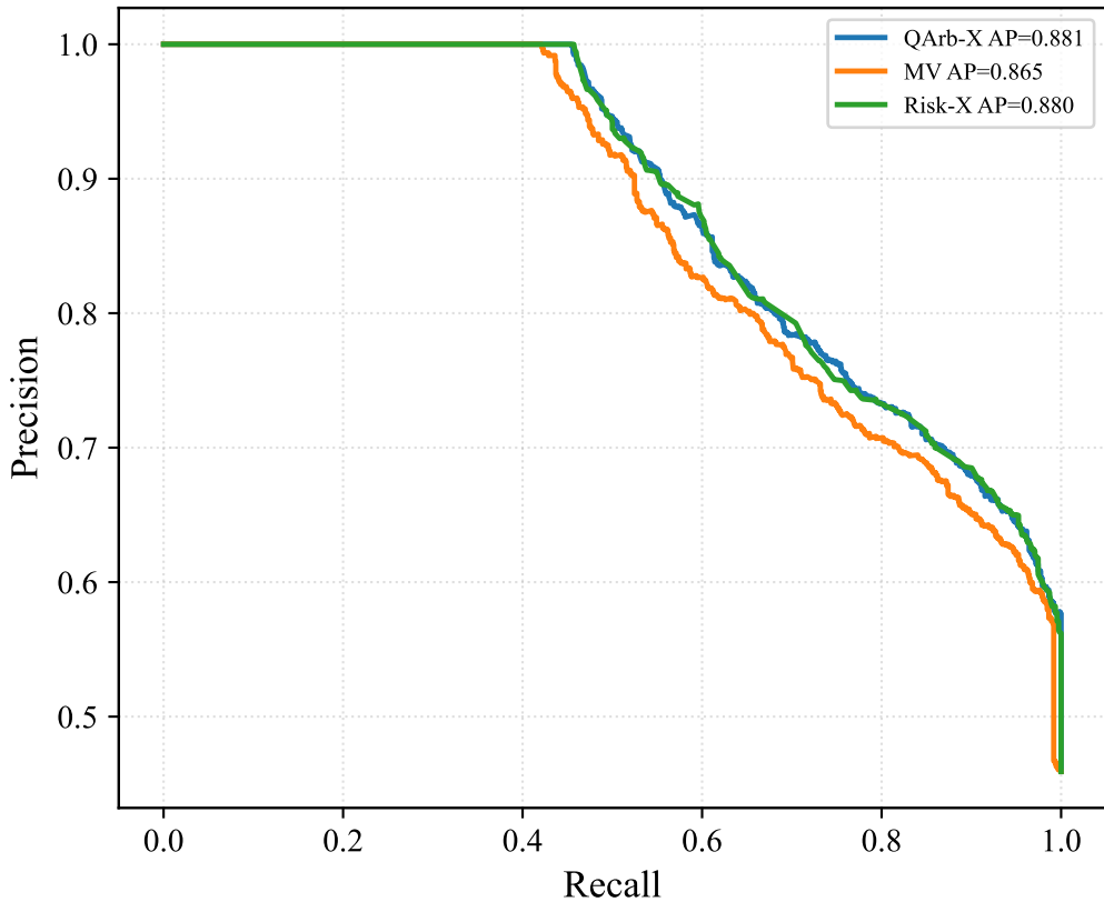
Agentic Precision-Recall Comparison
