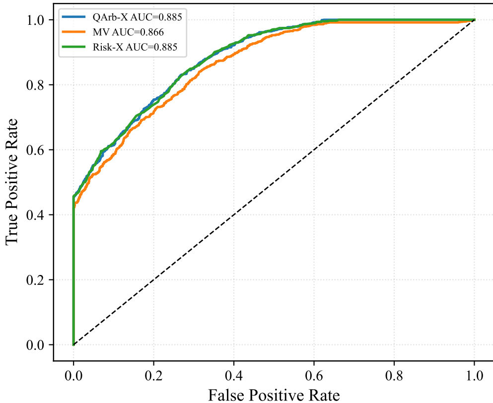
Agentic ROC Comparison
