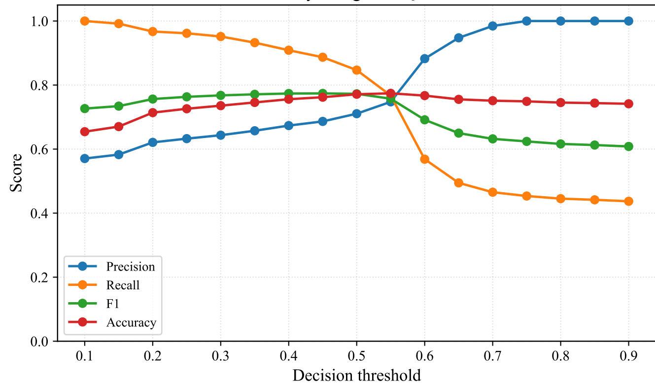
Threshold Sensitivity of Agentic Quantum Arbitration
