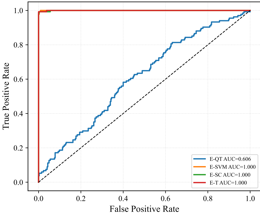
Email ROC Comparison
