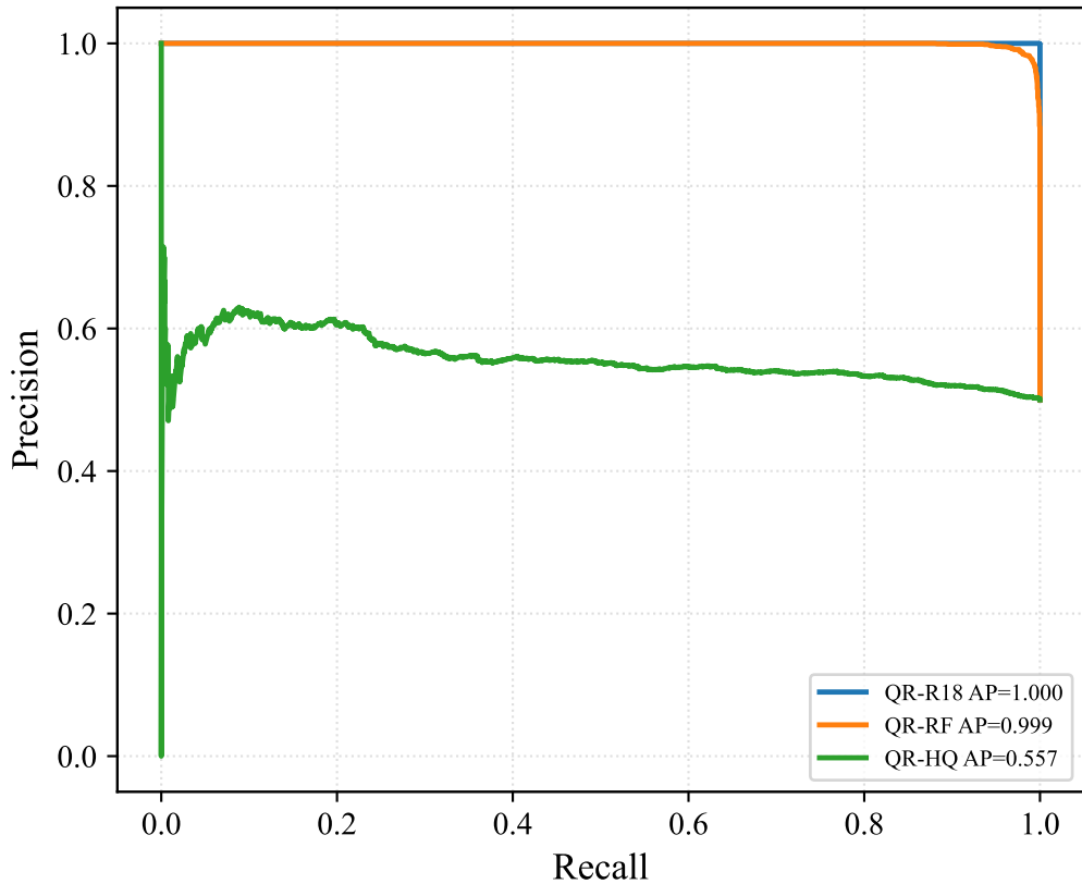
QR Precision-Recall Comparison
