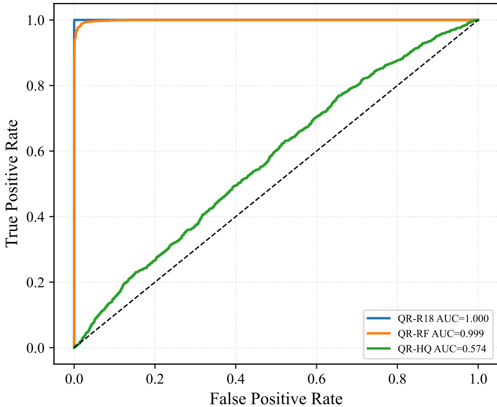
QR ROC Comparison
