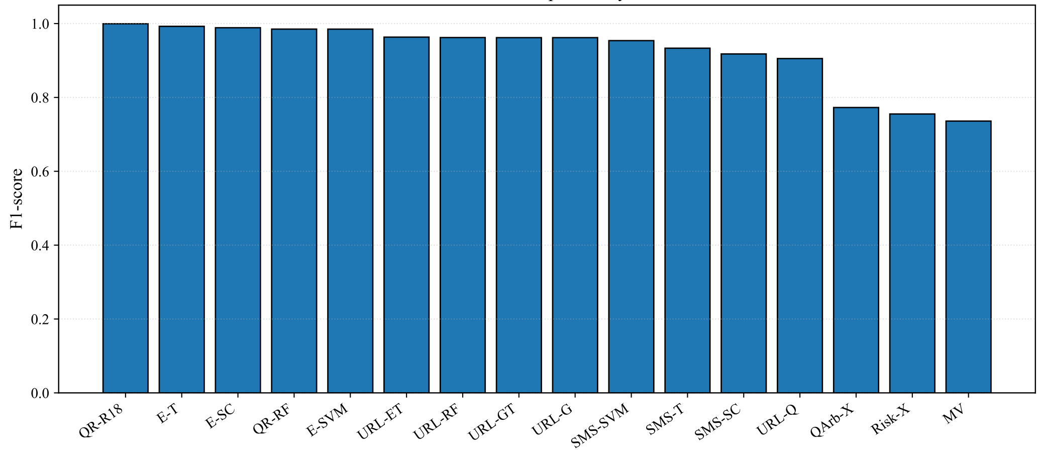
Ranked Model Comparison by F1-score
