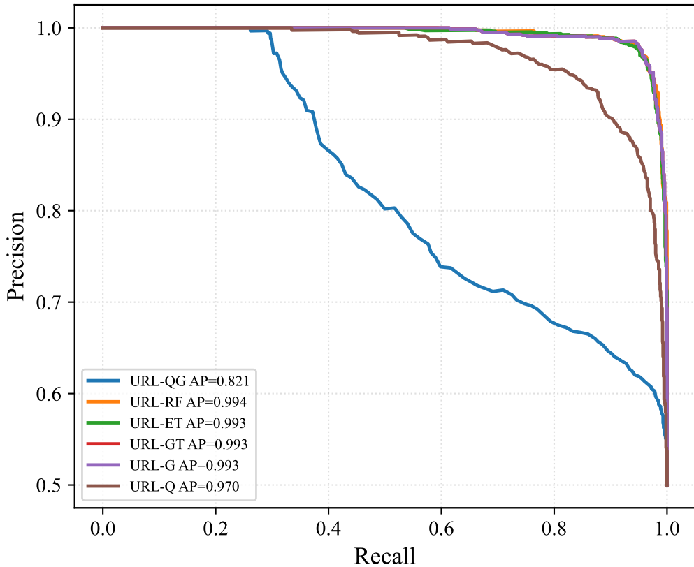
URL Precision-Recall Comparison
