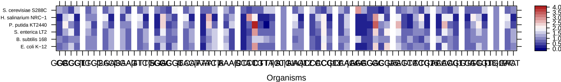
RSCU heatmap (codon usage vs synonymous expectation)
