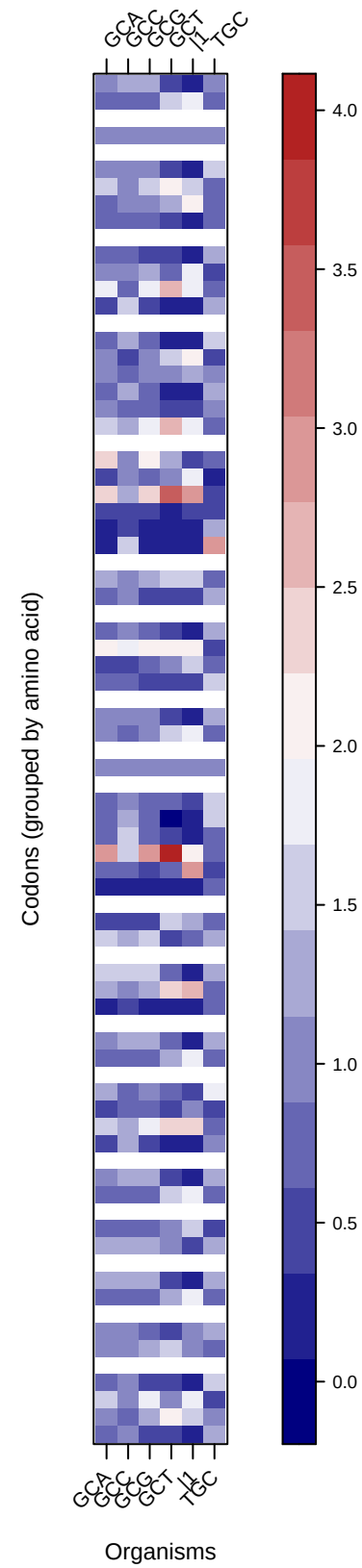
RSCU heatmap (codon usage vs synonymous expectation)
