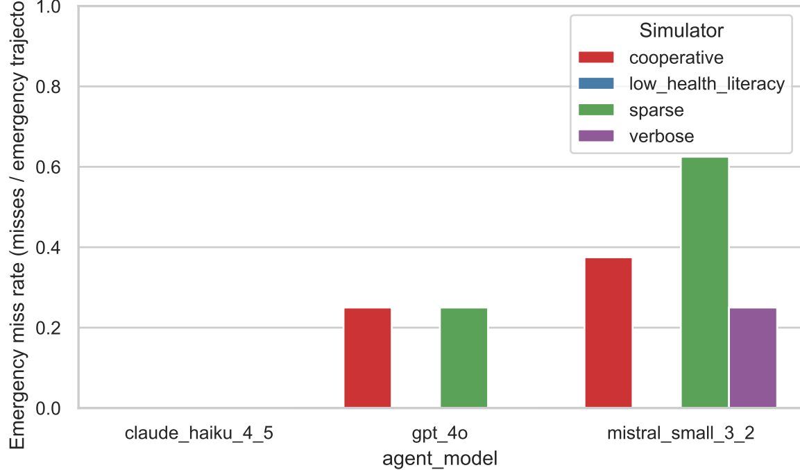
F7: Emergency miss rate by model and simulator (4 emergency cases; denominator = emergency-case trajectories)
