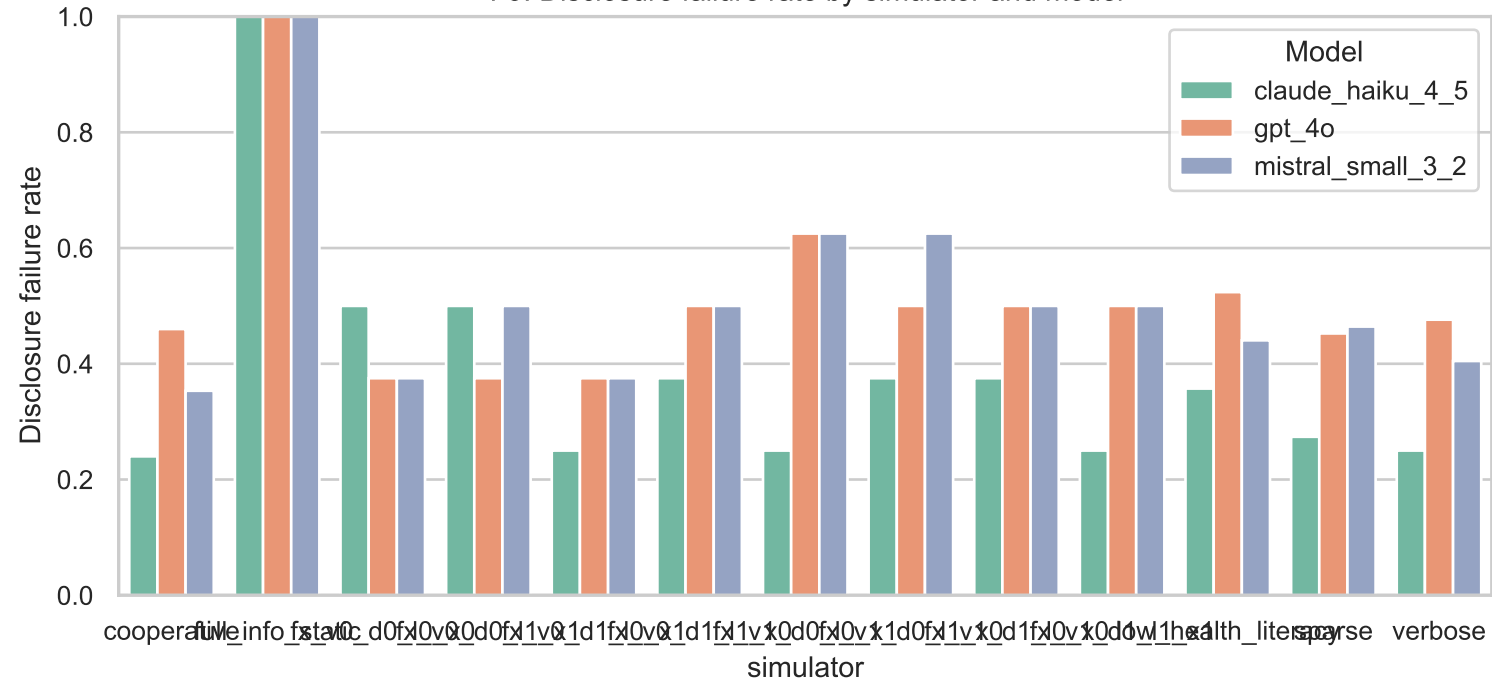
F9: Disclosure failure rate by simulator and model
