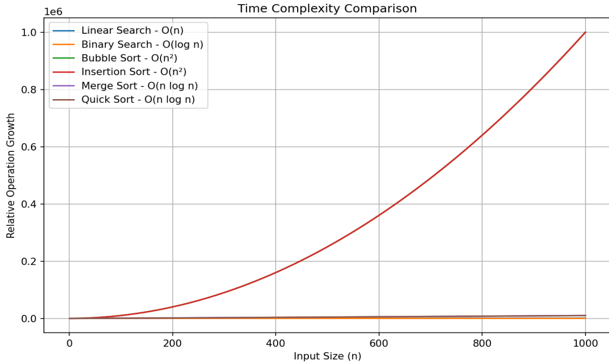
Time Complexity Comparison Graph (Linear Scale)
