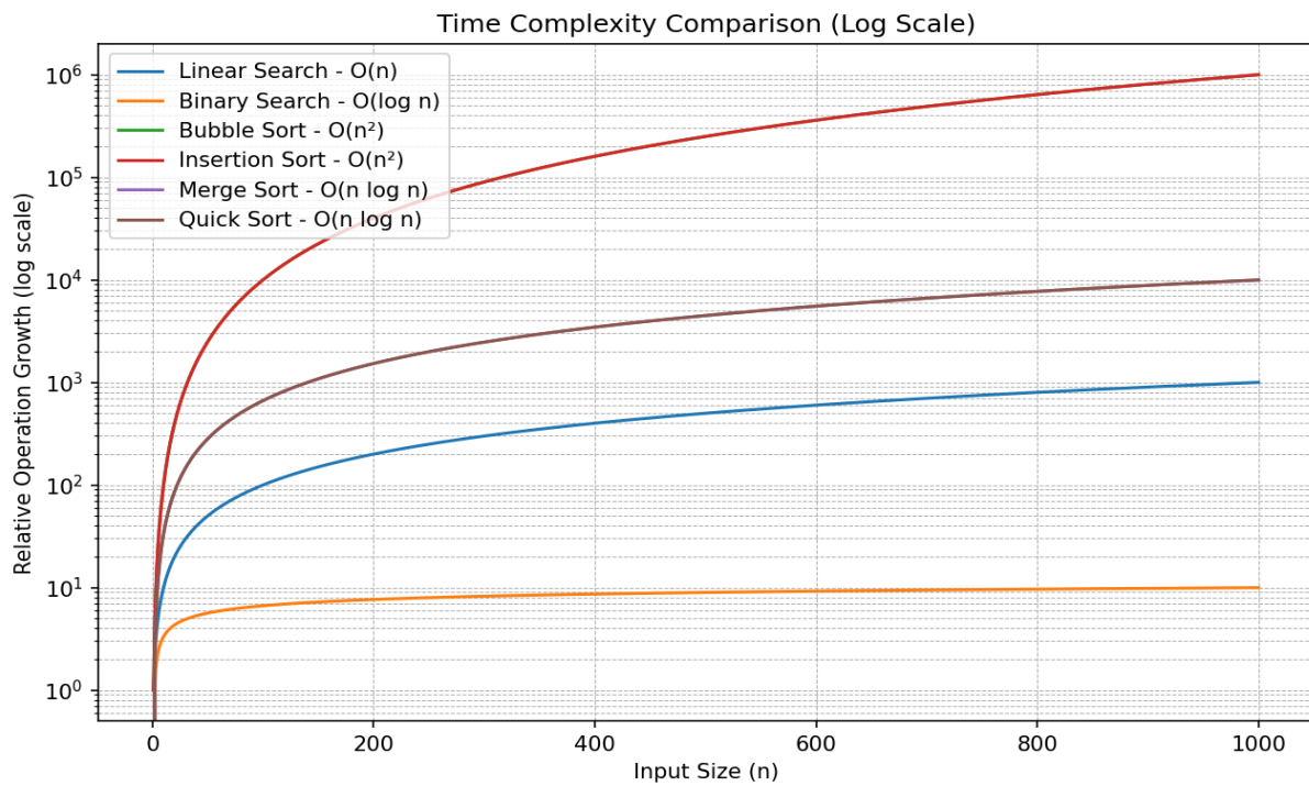
Time Complexity Comparison Graph (Log Scale)
