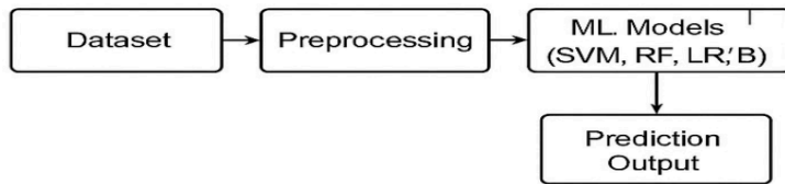
Figure 3.1: System Architecture
