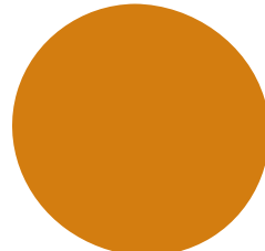
Full Moon
