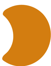
Quarter
