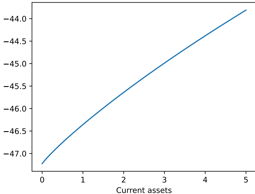
Efficiency 0.8, N=1000
