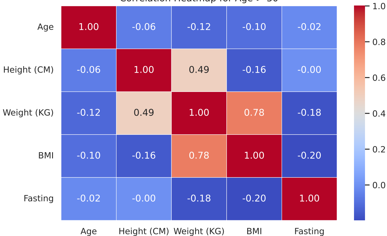
Correlation Heatmap for Age &gt; 30
