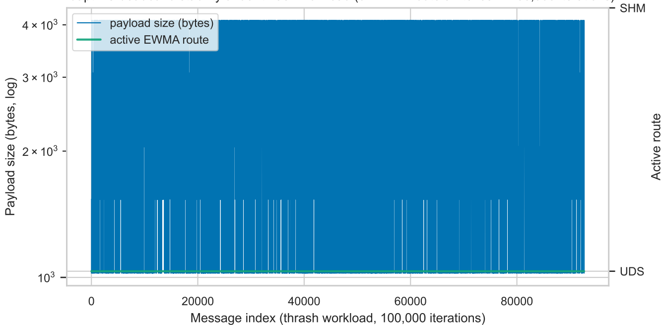
AdaptIPC deadband stability under thrash workload (0 EWMA route switches in 100,000 iterations)
