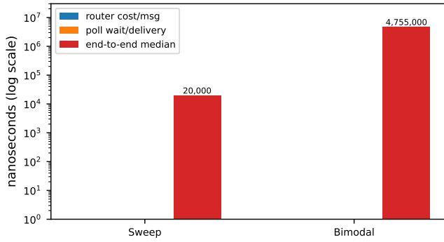
Fig. 7. Measured latency decomposition for the AdaptIPC engine (log scale) on the sweep and bimodal workloads, derived from in-process counters: per-message router cost (EWMA update + route decision), mean receiver poll wait per delivery, and median end-to-end latency. Component costs are two to three orders of magnitude below the end-to-end bimodal median, confirming that the residual latency is queueing delay behind buffered bulk traffic rather than per-message processing overhead.
