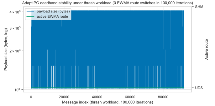
Fig. 6. AdaptIPC engine under the 100,000-iteration thrash workload. The dense vertical banding in the left-axis series is the per-message payload oscillation itself—each message alternates between 1024 B and 4096 B (with intermediate sizes) inside the deadband \Delta\tau = \tau_{\text{high}} - \tau_{\text{low}} = 3072 B; it does not indicate route changes. For rendering efficiency, consecutive duplicate payload-size samples are collapsed into single plotted steps; this collapsing is a plotting artifact only—some duplicates arise specifically because 4096 B frames exceed the datagram ceiling and are escalated from UDS to SHM without moving the sticky hysteresis state (Section IV-C)—and it is not evidence of route or payload change. The right-axis active-route line remains flat at UDS for the entire run: the EWMA state machine performs zero route switches (and hence zero false switches) over all 100,000 iterations, empirically validating the stability proof of Section III-D.
