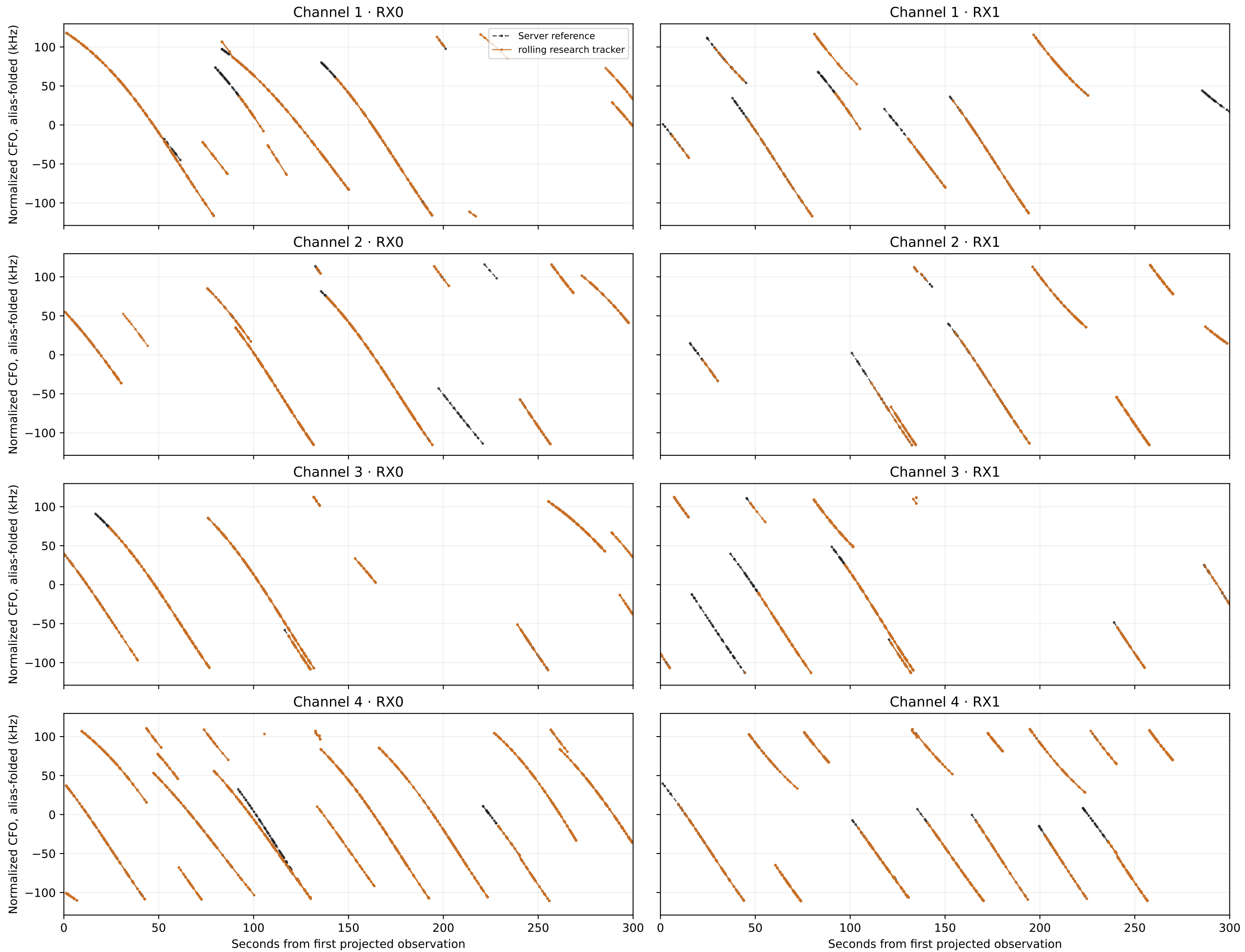
Full saved scan: server and ARM-derived tracks Measured GLRT CFO points assigned to tracks, joined in time; alias-wrap discontinuities are omitted.
