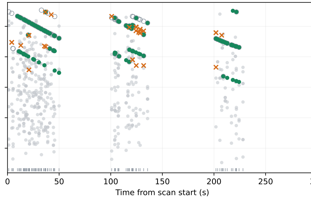
RX1: coarse cutoff removed — all evaluated 488 rejected by final GLRT; 192 pass
