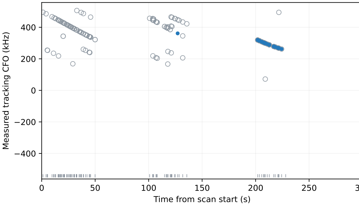
RX1: original cutoff 30 candidates pass final GLRT
