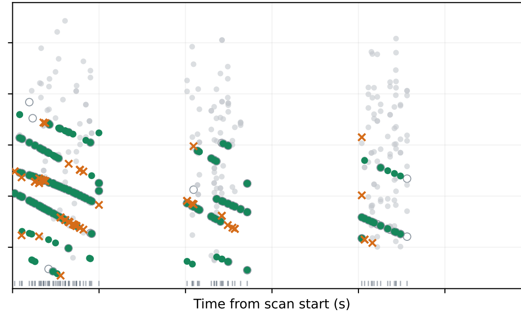
RX1: coarse cutoff removed — all evaluated 488 rejected by final GLRT; 192 pass
