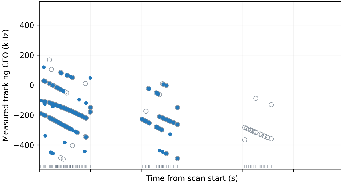
RX1: original cutoff 30 candidates pass final GLRT
