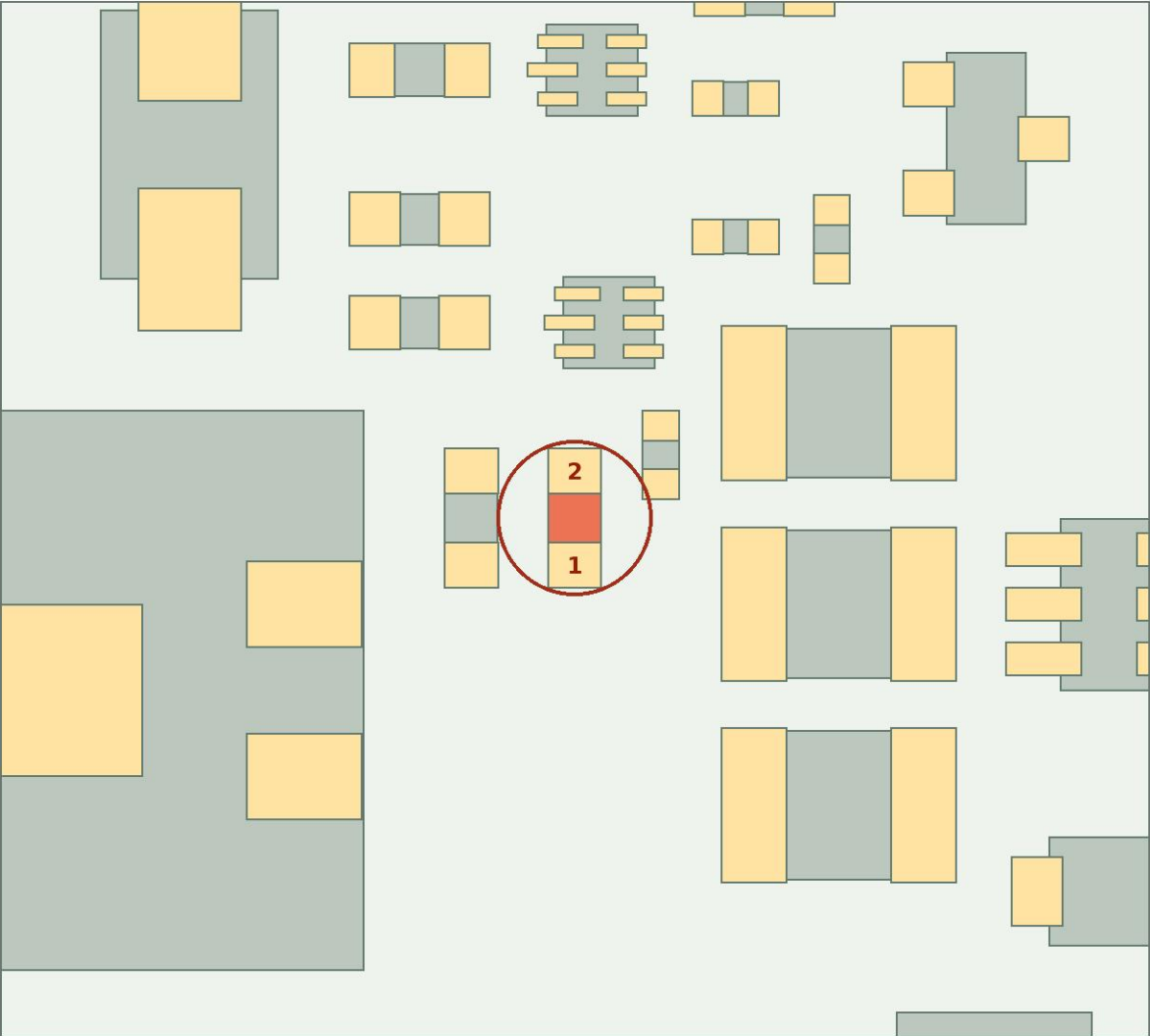
Exact target · highlighted body and numbered pads
