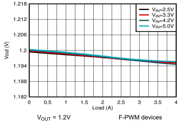
Figure 8-10. Load Regulation
