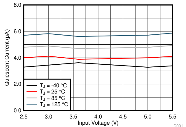
Figure 6-4. Quiescent Current
