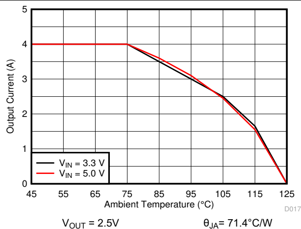
Figure 8-31. Thermal Derating
