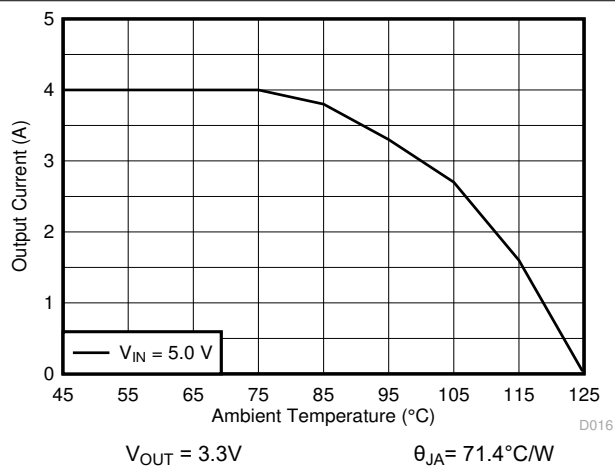
Figure 8-32. Thermal Derating
