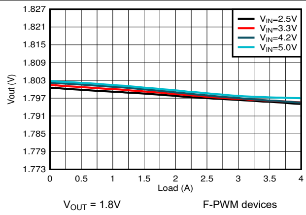
Figure 8-14. Load Regulation
