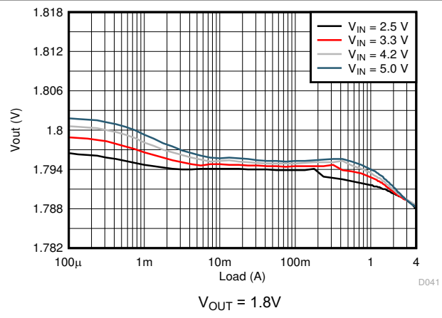
Figure 8-12. Load Regulation
