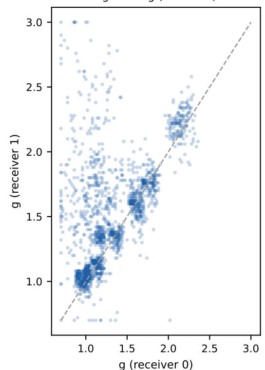
Fig. A2 — independent receivers agree on g (corr 0.64)
