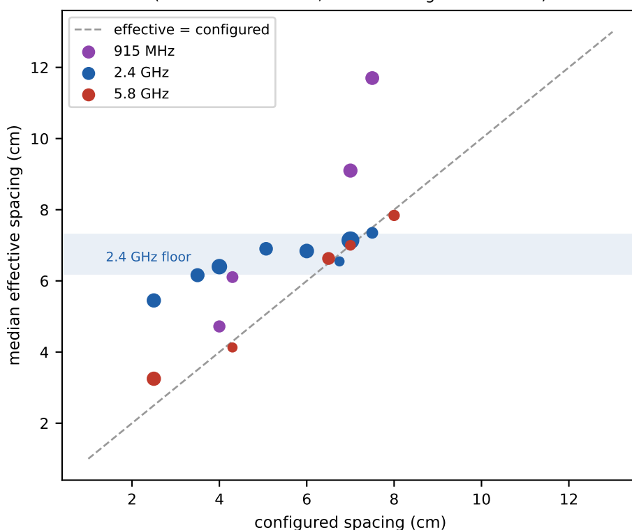
Fig. A1 — effective vs configured antenna spacing (marker size = # fits; bound-hitting fits excluded)
