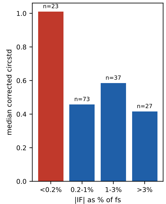
Fig. C2 — the cliff is the DC notch, not IF magnitude
