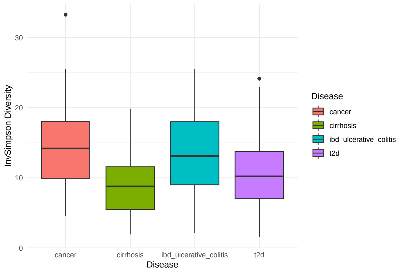
Alpha Diversity (InvSimpson)
