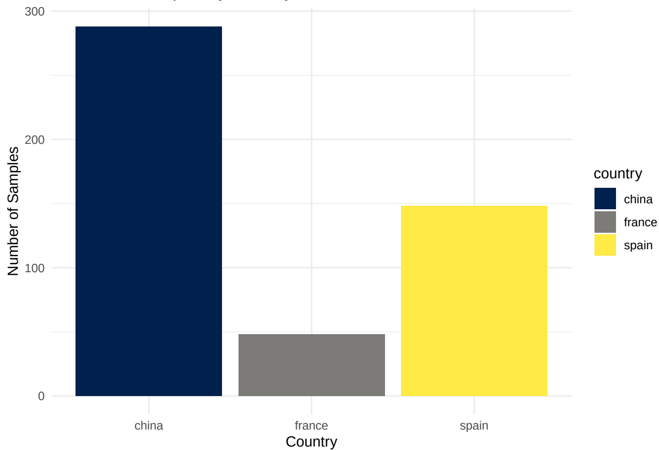
Number of Samples by Country
