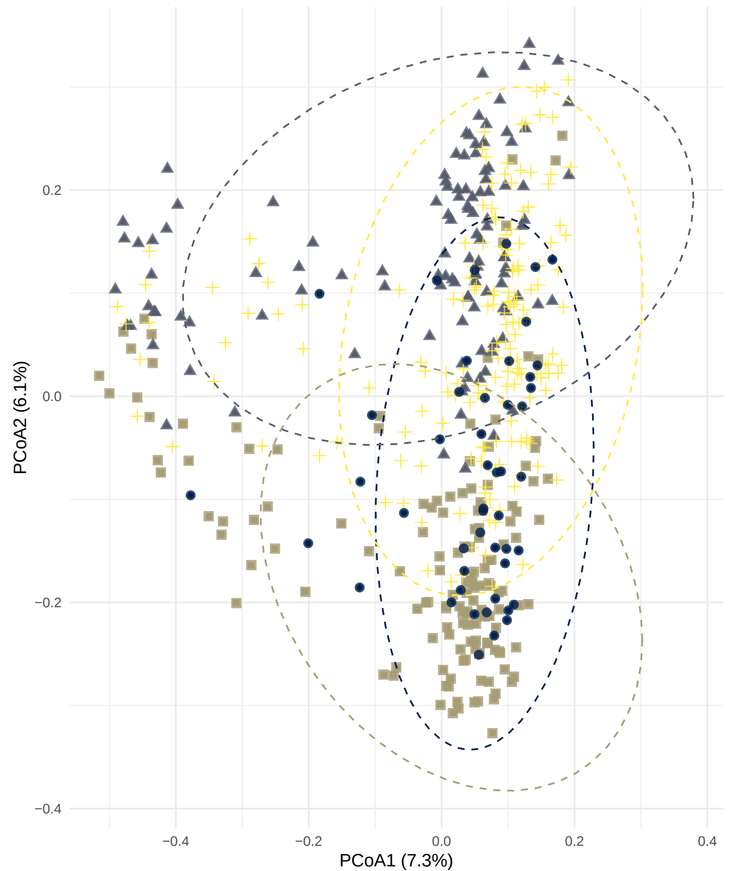
Jaccard Dissimilarity
