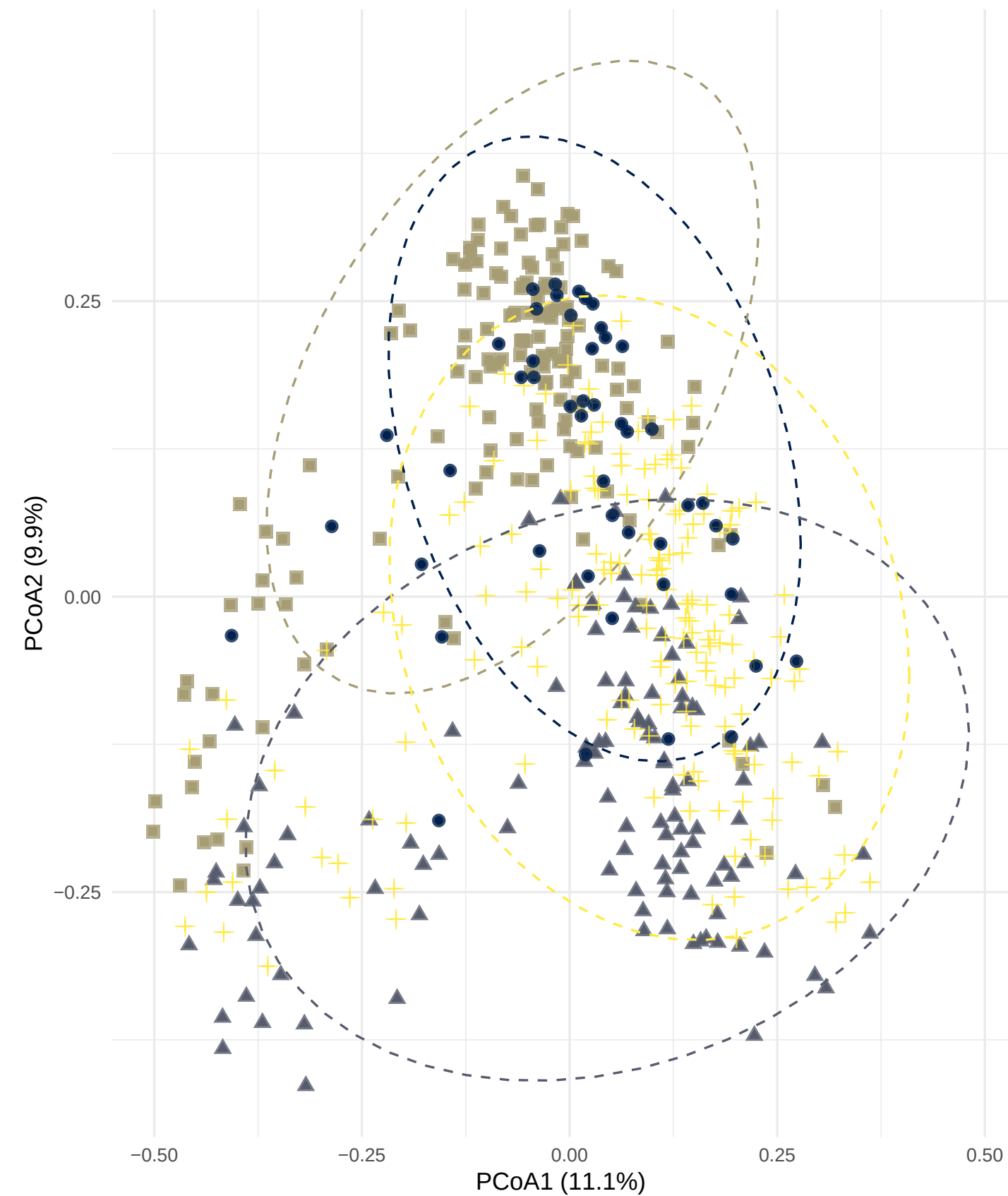
Bray–Curtis Dissimilarity
